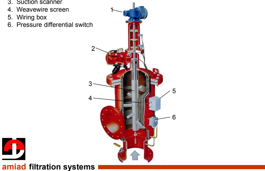
Figure 1: Amiad Model EBS Automatic Strainer
